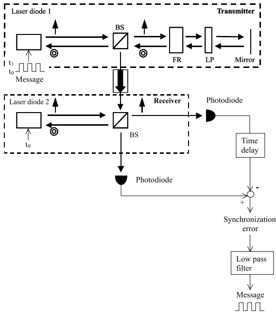
Fig. 7. Schematic representation of the secure communication scheme we propose. The message encoding is achieved by chaos shift keying, i.e., the bit stream modulates the transmitter diode injection current.
