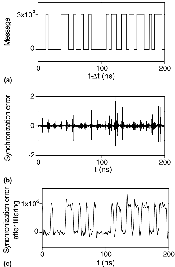
Fig. 8. Numerical simulations, (a) 250 Mbit/s input message, (b) synchronization error before filtering, (c) synchronization error after filtering.
